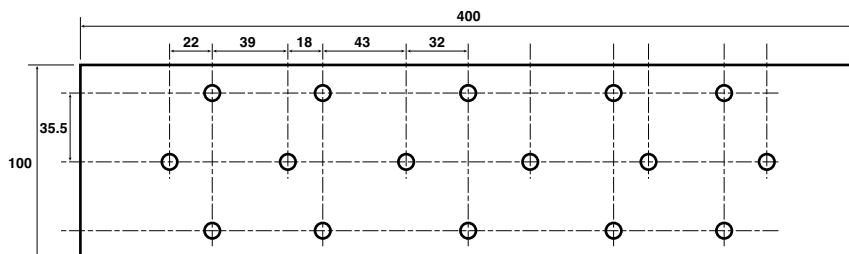
FOS-400 Series
